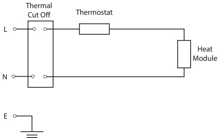
Electric Wiring Diagram
